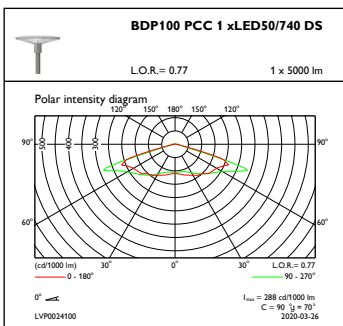
OFPC1_BDP100PCC1xLED50740DS
