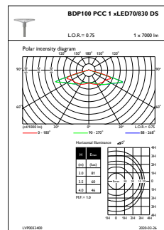
OFPL1_BDP100PCC1xLED70830DS
