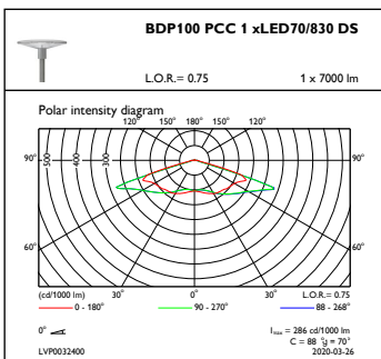
OFPC1_BDP100PCC1xLED70830DS
