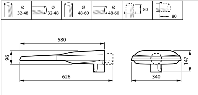
BGP283 LED100-4S/740 I DM50 D9 48/60S
