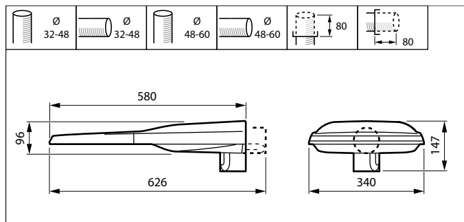
BGP293 LED100-4S/740 II DM11 CLO S05Z1Z1
