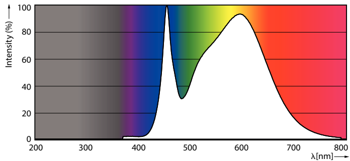
LEDForce HPI 140W Others E40 840 1
