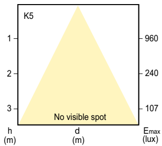
LDBE_IREFESP_60W_NR63_30D-Beam diagram
