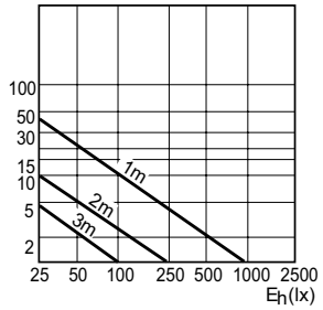
LDAC_IREFESP_60W_NR63_30D-Accent diagram
