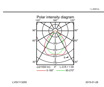
IFPC_4MX900 G3 491 1xLED40S/830 PSU WB-Polar Indoor (combined)
